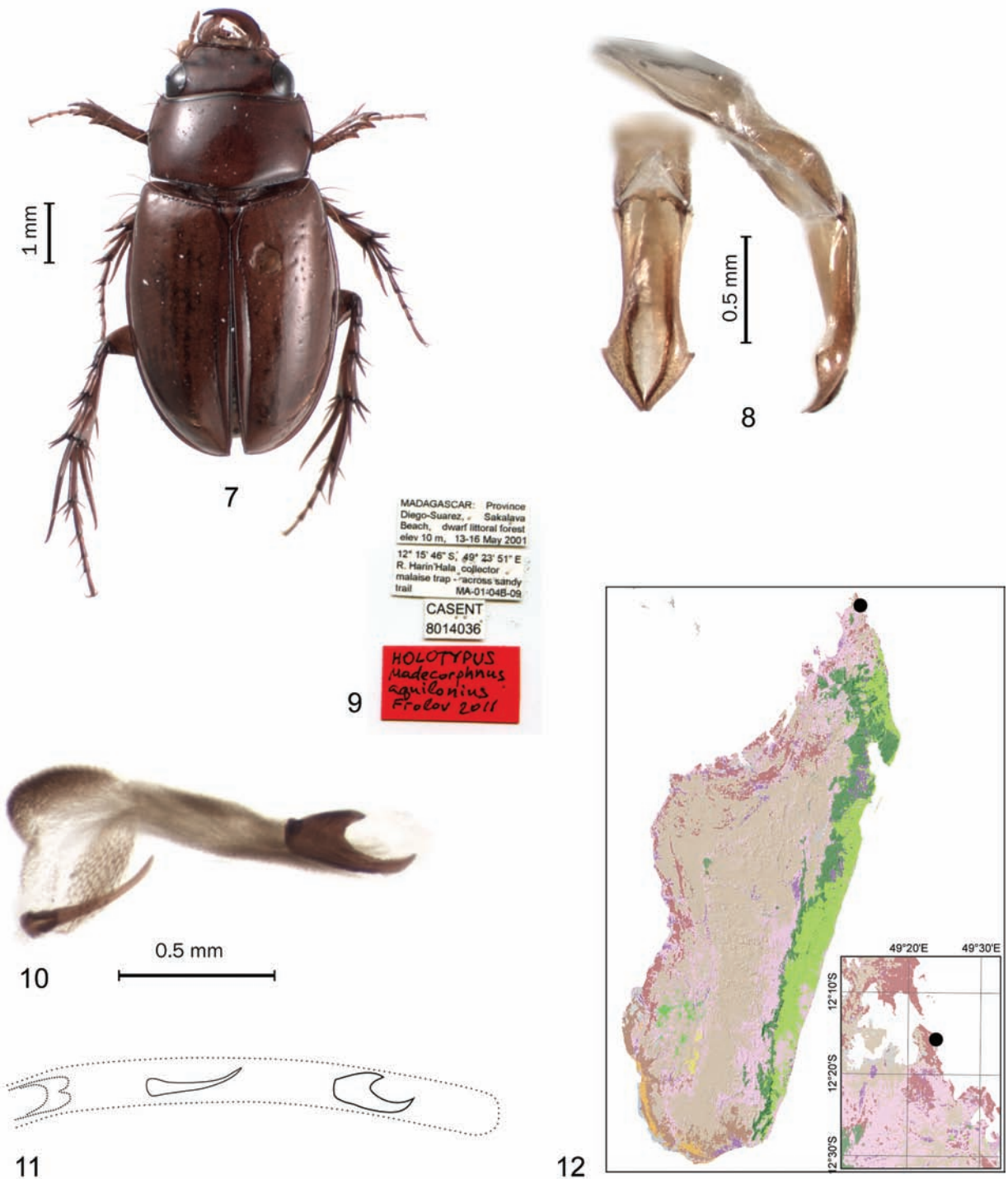
Figs 7–12. Madecorphnus aquilonius sp. nov., holotype, male: 7 – habitus; 8 – parameres in dorsal and lateral view; 9 – labels; 10 – invaginated internal sac of aedeagus; 11 – schematic representation of armature of invaginated internal sac; 12 – distribution map (see Fig. 6 for legend).
