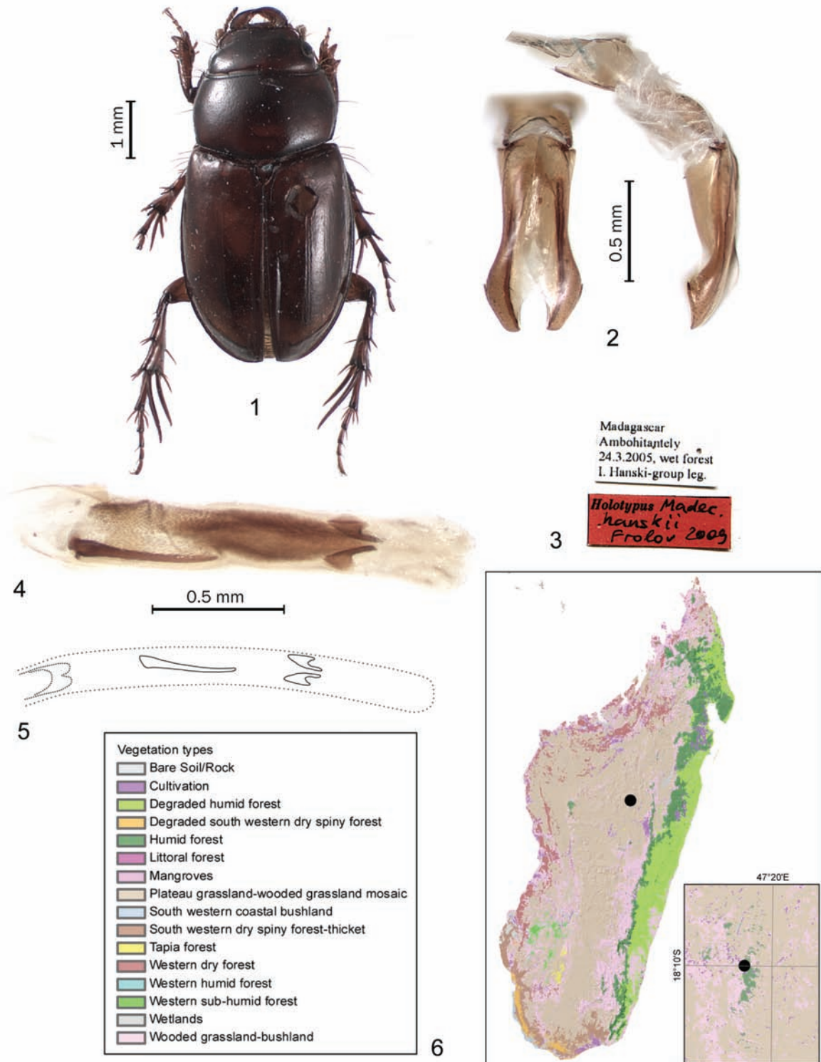
Figs 1–6. Madecorphmus hanskii sp. nov., holotype, male: 1 – habitus; 2 – parameres in dorsal and lateral view; 3 – labels; 4 – invaginated internal sac of aedeagus; 5 – schematic representation of armature of invaginated internal sac; 6 – distribution map and a legend to vegetation types.
